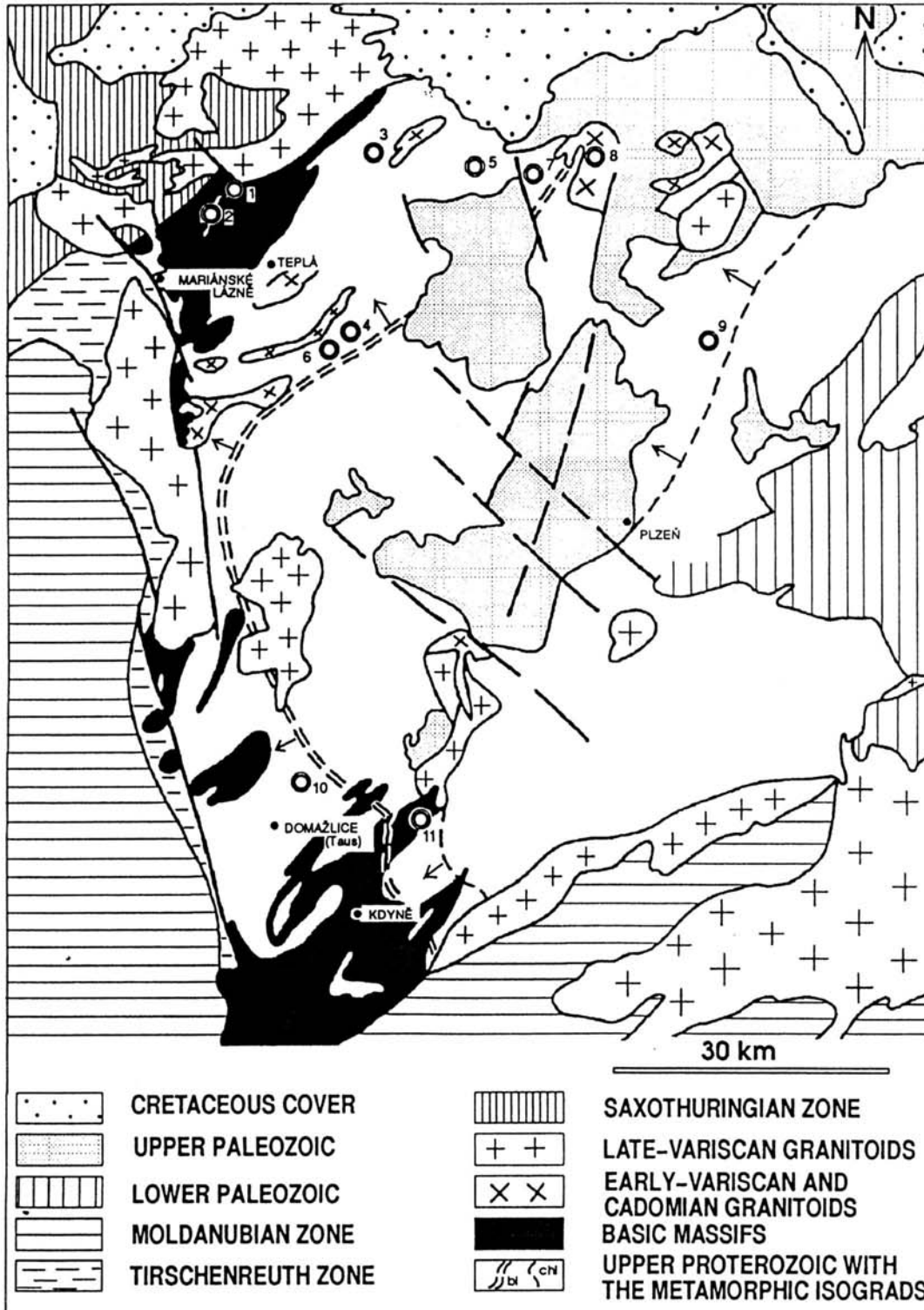
Figure 1. Generalized geological map of the Teplá-Barrandian Zone indicating locations sampled for ^{40}\text{Ar}/^{39}\text{Ar} dating.
