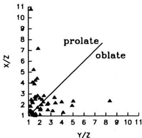
Fig. 1. Flinn diagram of 50 strain analyses in amphibolites of the Bavarian part of the GAM
