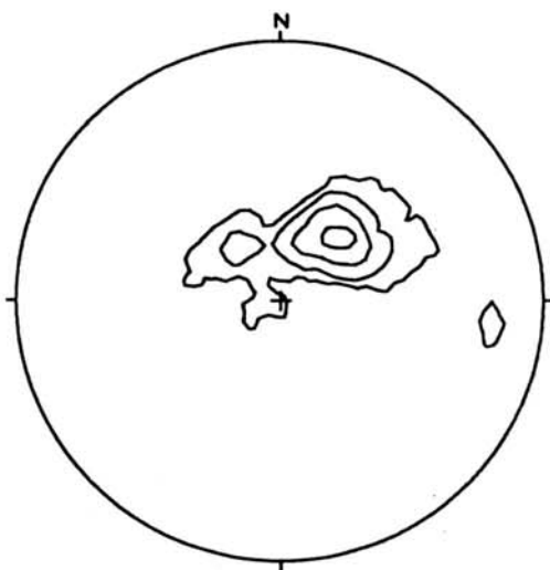
Fig. 2a: 201 Mineral stretching lineations, Bavarian part of GAM, equal area net, lower hemisphere, 2–5–10–20%
