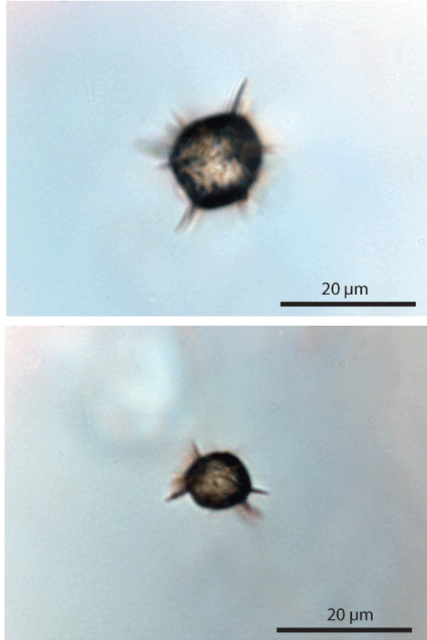
Figure S1: Rounded metamict zircon inclusions in quartz of the sodic banded aplite.
