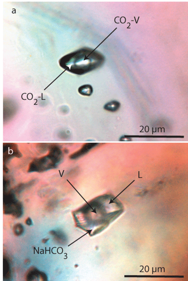
Figure S2: Fluid inclusions in quartz of the sodic banded aplite from Roncadeira, carbonic ( a ) and aqueous with nahcolite daughter crystals ( b ).
