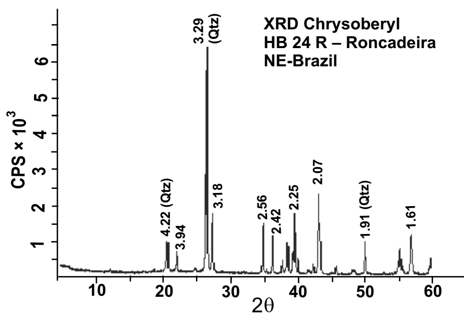
Figure S3: X-ray diffraction pattern of the Roncadeira chrysoberyl and minor quartz.
