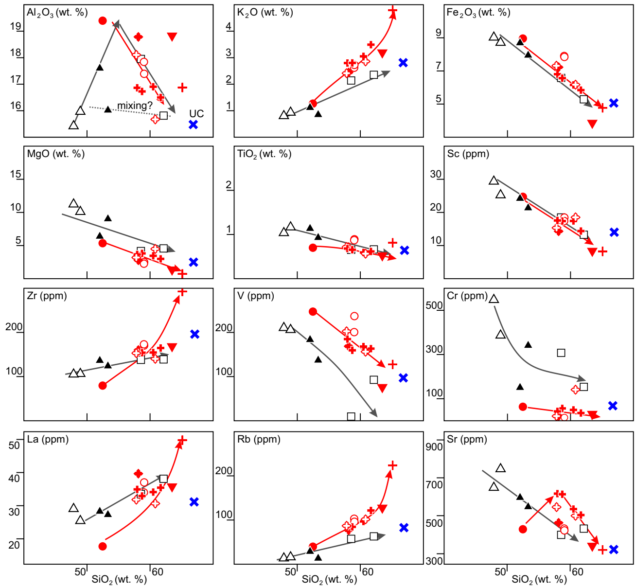
ESM4 - Multiple binary diagrams with \text{SiO}_2 vs. selected major oxide and trace element concentrations. Possible fractionation trends are represented by red and black arrows. UC: Upper crust (Rudnick and Gao, 2003).
