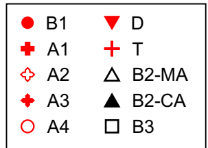
ESM4 - Multiple binary diagrams with \text{SiO}_2 vs. selected major oxide and trace element concentrations. Possible fractionation trends are represented by red and black arrows. UC: Upper crust (Rudnick and Gao, 2003).
